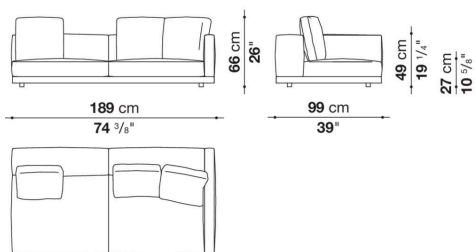
DBL189TD
