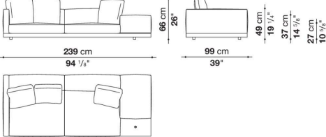
DB239D_2
