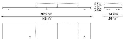
DBL370PS
