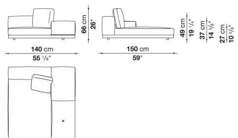
DBL150LD_2
