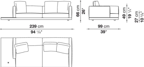
DB239S_1
