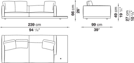
DB239D_1
