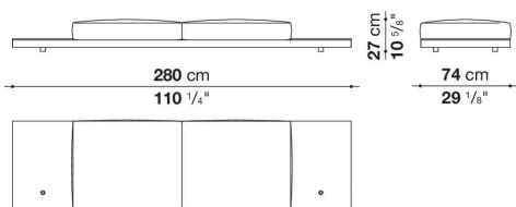
DBL280P
