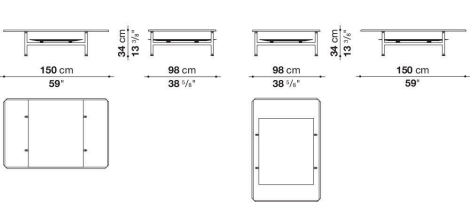
TDS150
