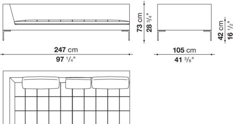
CHL247S_1Q
