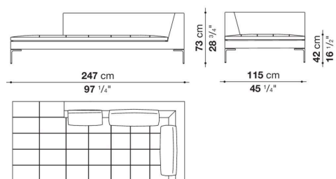
CHL247LS_1Q
